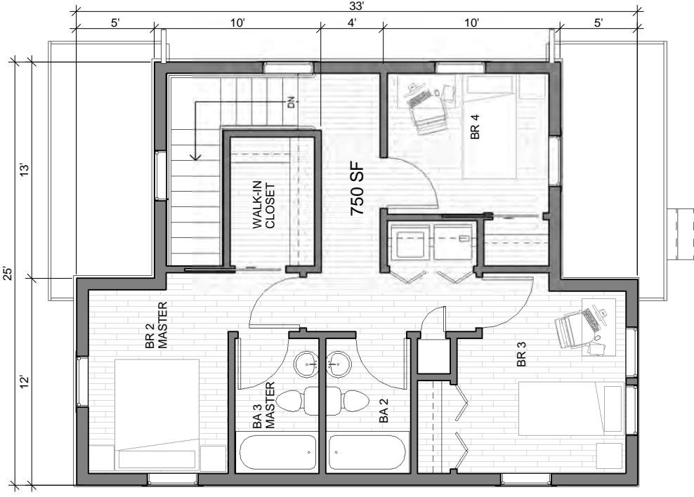
② 4BR - SECOND FLOOR PLAN 1/4" = 1'-0"
