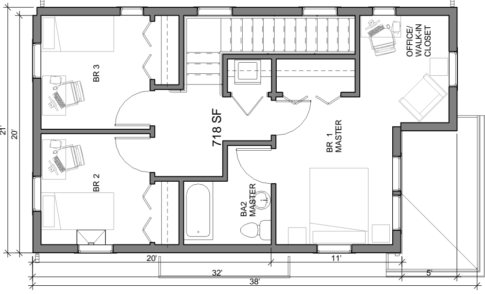
② 3BR - SECOND FLOOR PLAN 1/4" = 1'-0"
