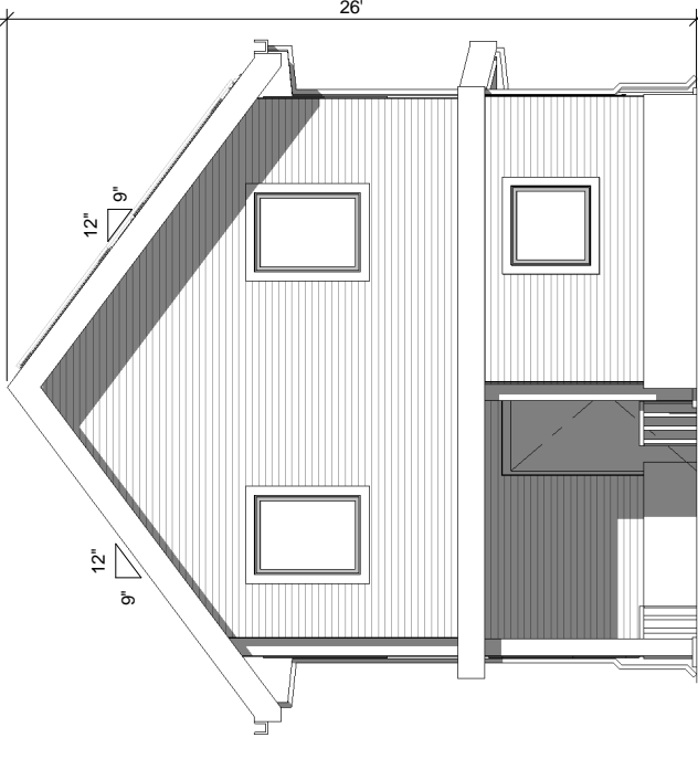
⑤ 3BR - REAR ELEVATION 1/4" = 1'-0"
