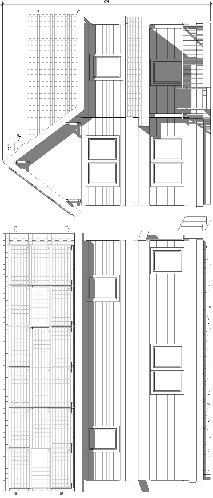
⑤ 4BR - ELEVATION_SIDE 1 1/4" = 1'-0"
