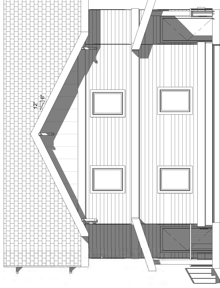
⑥ 4BR - ELEVATION_SIDE 2 1/4" = 1'-0"
