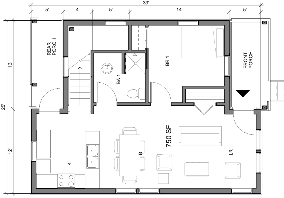
① 4BR - FIRST FLOOR PLAN 1/4" = 1'-0"
